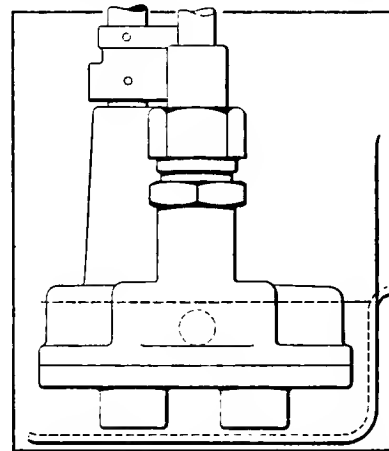
Fig. 4—Exterior of gear pump often used in connection with force-feed oiling
